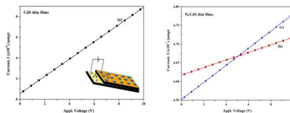
Figure 4: The I-V plots of Cd_{1-x}Ni_xS thin films for (a) x = 0 , (inset: schematic view of the device) (b) x = 0.04 and (c) x = 0.08 M
