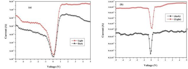
Figure 5: Forward and reverse bias I-V measurements of (a) x=0 and (b) x=0.08 M, Ni doped CdS hybrid heterojunction photodiodes under dark and under illumination.
