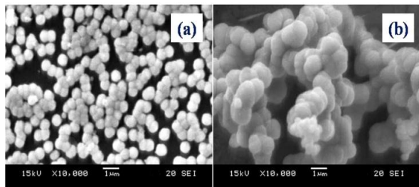
Figure 2 (a, b): SEM images of Cd_{1-x}Ni_xS ( x = 0 and 0.08 M).
