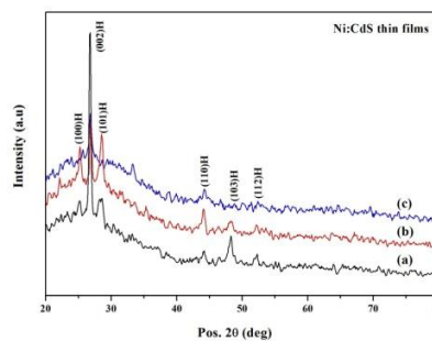
Figure 1: X – ray diffraction pattern of \text{Cd}_{1-x}\text{Ni}_x\text{S} thin films obtained at various Ni concentrations (a) x = 0 , (b) x = 0.04 and (c) x = 0.08 \text{ M} .
