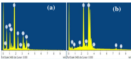
Figure 3 (a, b): EDX spectra of Cd_{1-x}Ni_xS ( x = 0 and 0.08 M).
